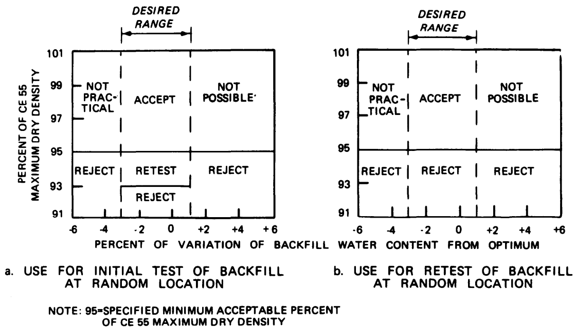
Figure 7-1. Acceptance Rejection Scheme for a Backfill Area.
